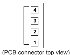
Figure 2-2. J901 and J900 Pin Numbers
