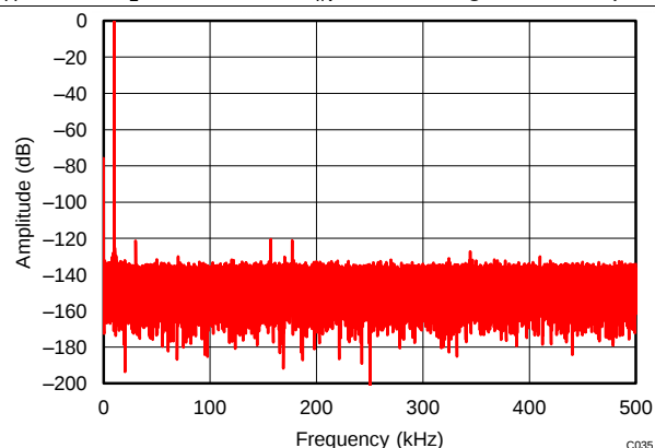
Figure 31. Typical FFT Plot
