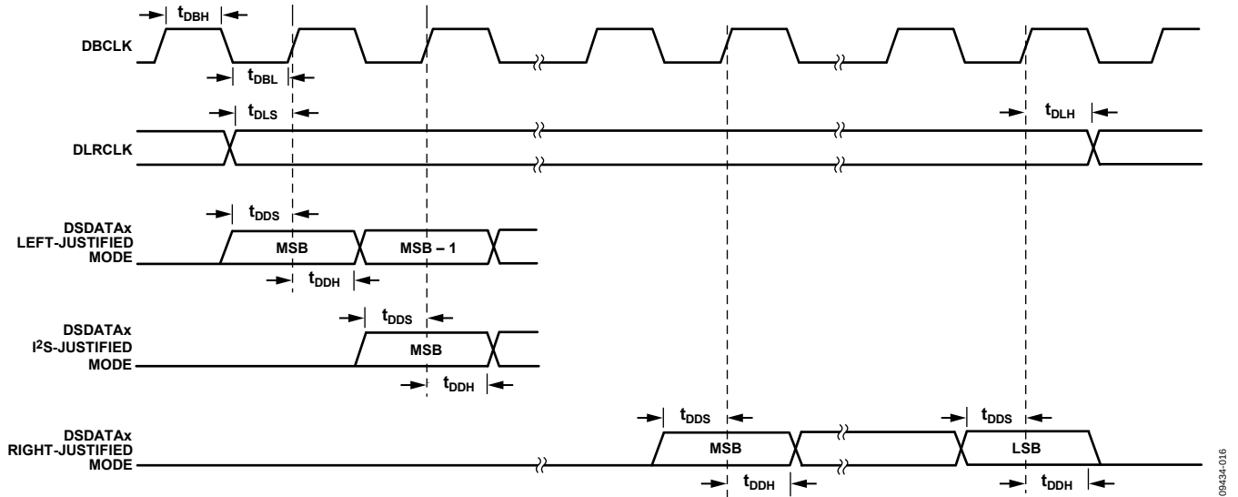
Figure 16. DAC Serial Timing
