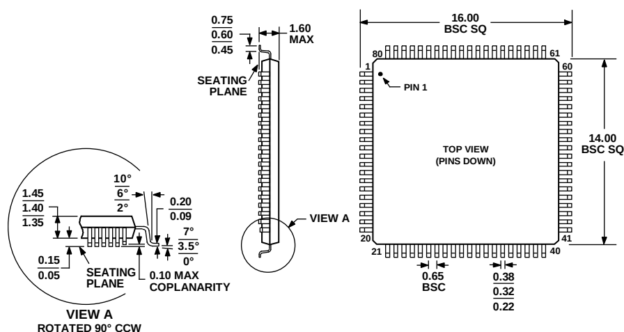
Figure 19. 80-Lead Low Profile Quad Flat Package [LQFP] (ST-80-2) Dimensions shown in millimeters
