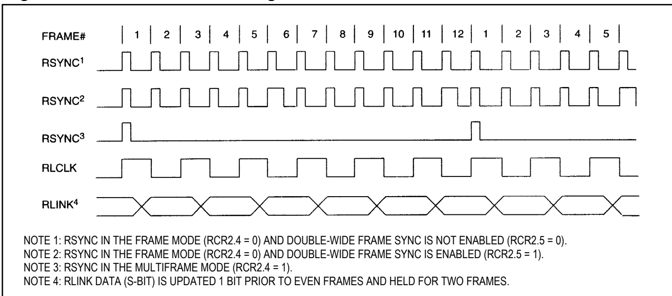
Figure 14-1. Receive Side D4 Timing
