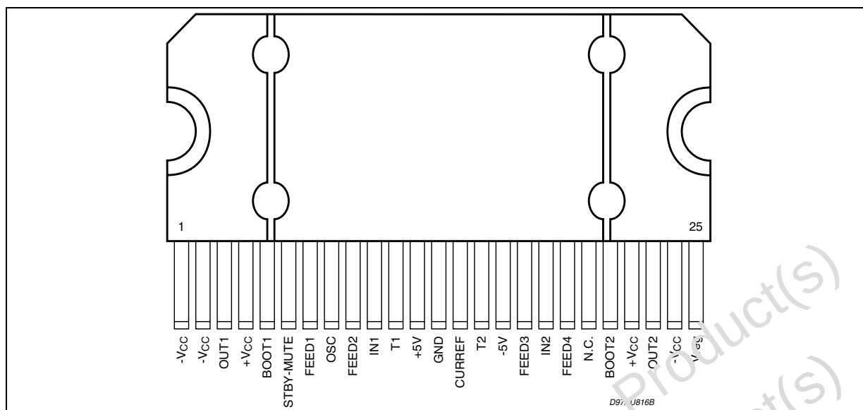
Figure 4. Pin Connection
