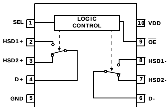
ISL54222A (10 LD MSOP) TOP VIEW
