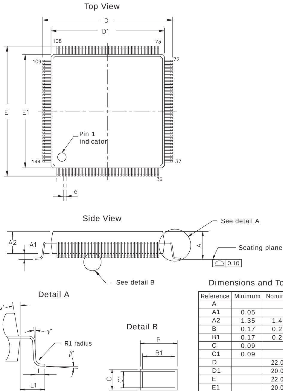
Figure 12. Package Drawing
