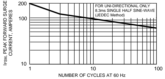
FIG. 6 - MAXIMUM NON-REPETITIVE PEAK FORWARD SURGE CURRENT
