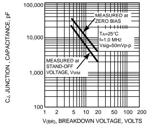
FIG. 4 - TYPICAL JUNCTION CAPACITANCE UNI-DIRECTIONAL TYPE
