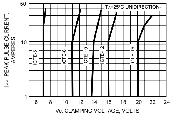
FIG. 7 - TYPICAL CHARACTERISTIC CLAMPING VOLTAGE
