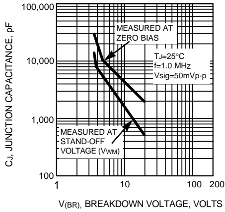
FIG. 5 - TYPICAL JUNCTION CAPACITANCE BIDIRECTIONAL TYPE
