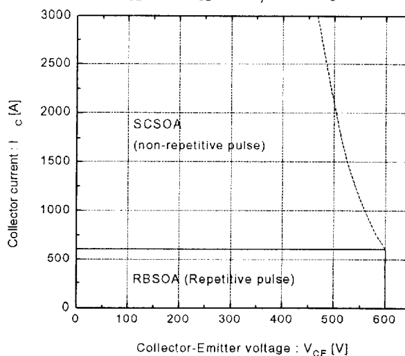
Reversed biased safe operating area +V_{GE}=15V , -V_{GE}\leq 15V , T_J\leq 125^\circ C , R_G\geq 6.8\Omega
