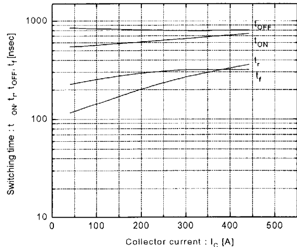
Switching time vs. Collector current V_{CC}=300\text{V} , R_G=6.8\Omega , V_{GE}=\pm 15\text{V} , T_j=125^\circ\text{C}
