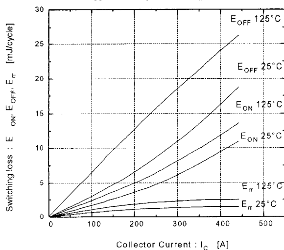
Switching loss vs. Collector current
