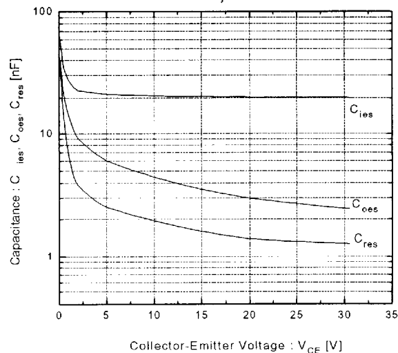
Capacitance vs. Collector-Emitter voltage
