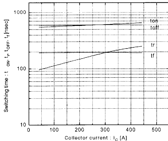
Switching time vs. Collector current V_{CC}=300\text{V} , R_G=6.8\Omega , V_{GE}=\pm 15\text{V} , T_j=25^\circ\text{C}
