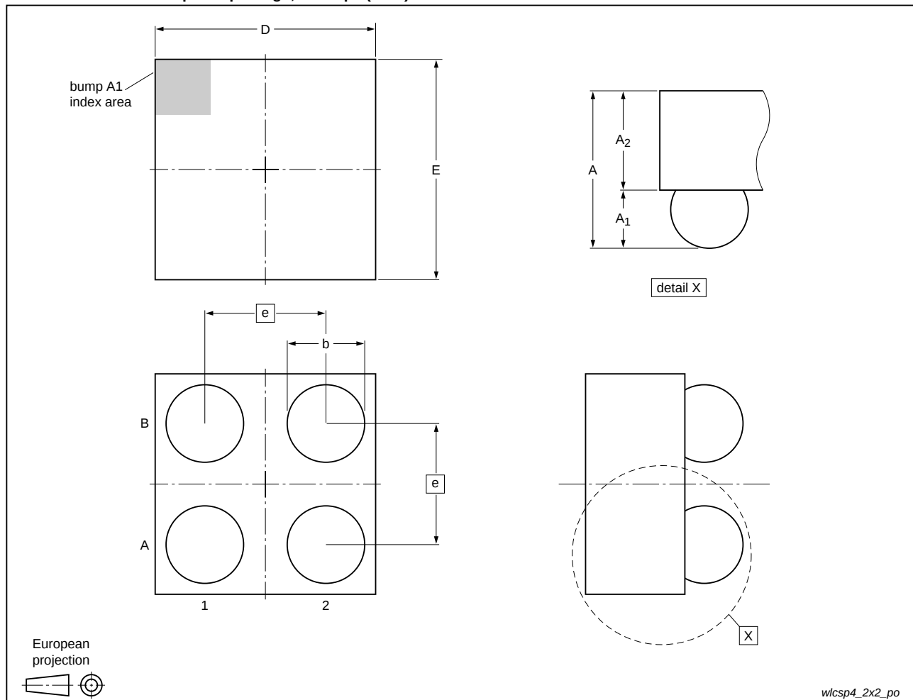
Fig 35. Package outline WLCSP4
