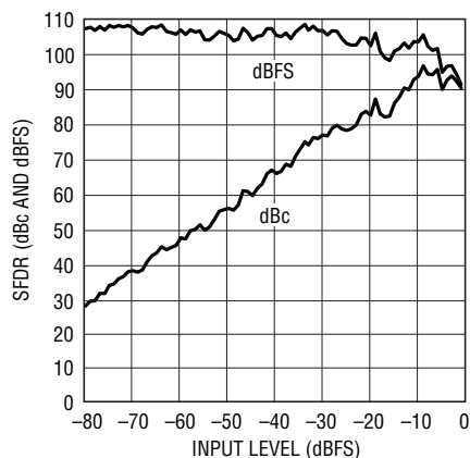
LTC2257-14: SFDR vs Input Level, f_{IN} = 70\text{MHz} , 2\text{V} Range, 40\text{Mps}
