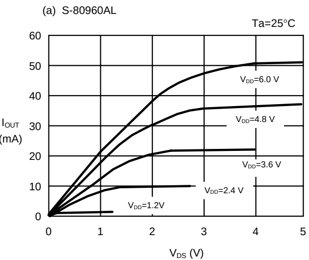
(5) Nch transistor output current ( I_{OUT} ) - V_{DS}
