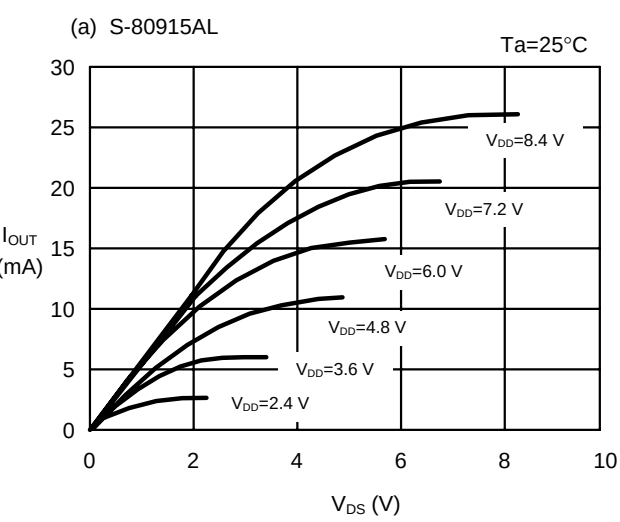
(6) Pch transistor output current ( I_{OUT} ) - V_{DS}
