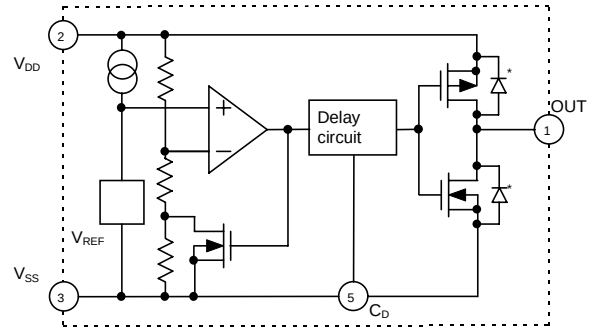
(2) CMOS active low output
