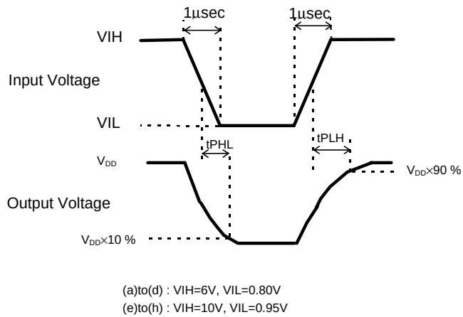
Figure 18 Measuring conditions of response time
