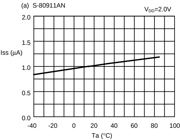
(4) Current consumption ( I_{SS} ) - Temperature ( T_a )
