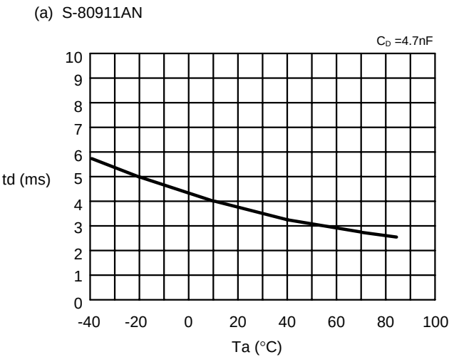
(12) Delay time (tpd) - Temperature (Ta)
