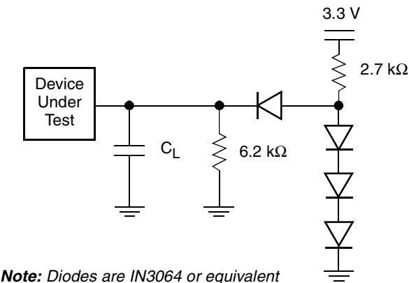
Figure 12. Test Setup
