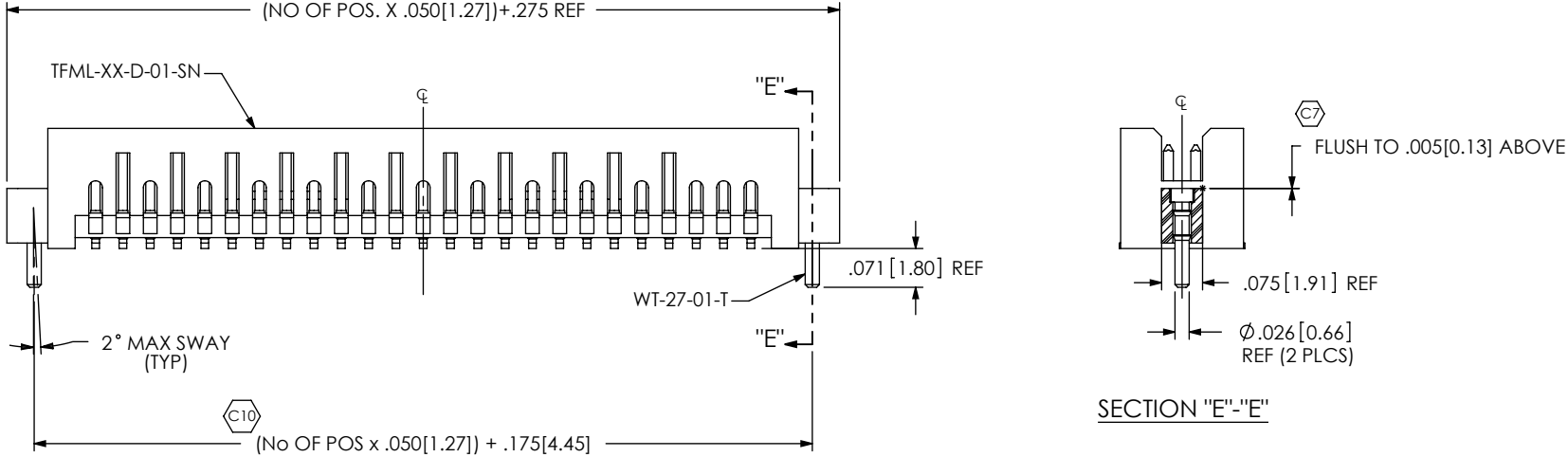
FIG. 10 -SN: SOLDER PIN OPTION (SHOWN: TFML-125-02-XXX-D-SN) (SAME AS FIG. 1, UNLESS OTHERWISE STATED) (ONLY AVAILABLE ON -02 LEAD STYLE)
