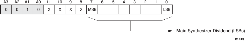
Figure 8. Main Dividend LSB Register (Write Only)
