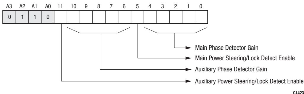
Figure 12. Phase Detector/Charge Pump Control Register (Write Only)
