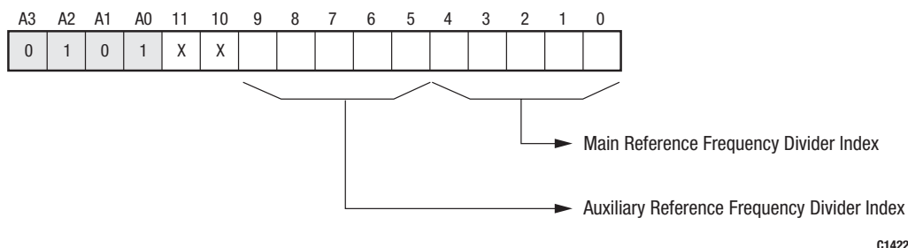
Figure 11. Reference Frequency Dividers Register (Write Only)
