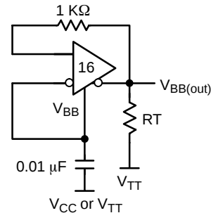
Figure 8. V BB Voltage Reference Generator
