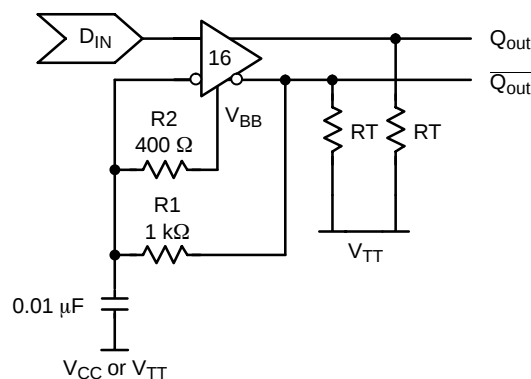
Figure 18. Schmitt Trigger with 228 mV Hysteresis
