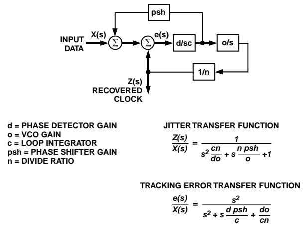
Figure 13. PLL/DLL Architecture
