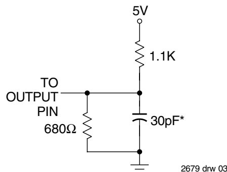
Figure 1. Output Load
