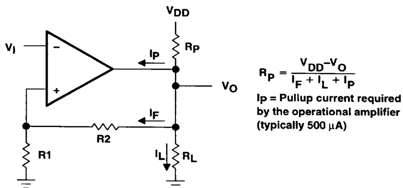
Figure 113. Resistive Pullup to Increase V_{OH}
