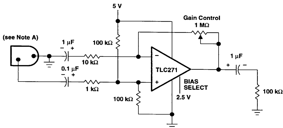
Figure 122. Microphone Preamplifier
