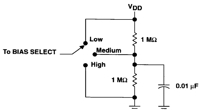
Figure 106. Bias Selection for Single-Supply Applications
