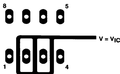
Figure 101. Isolation Metal Around Device inputs (JG and P packages)
