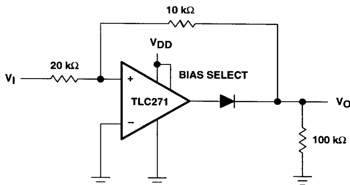
Figure 127. Full-Wave Rectifier
