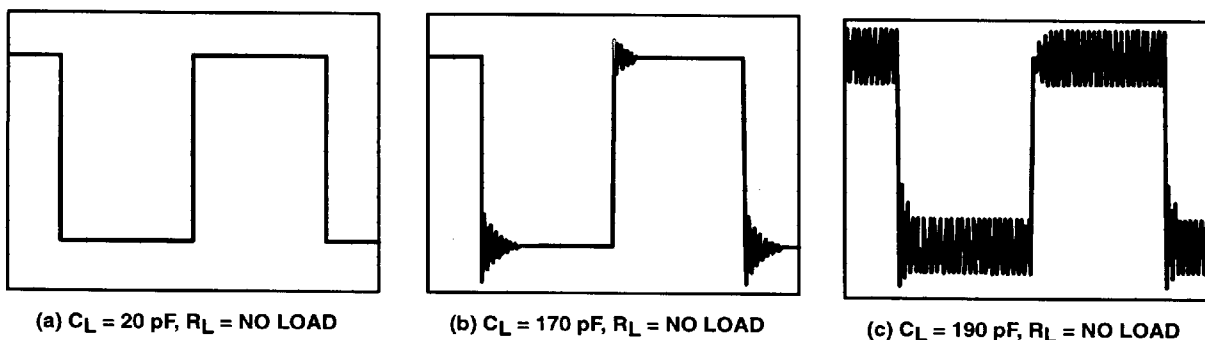
Figure 111. Effect of Capacitive Loads in Medium-Bias Mode
