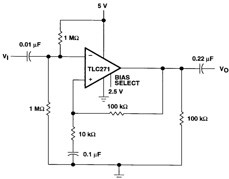
Figure 121. Single-Supply AC Amplifier
