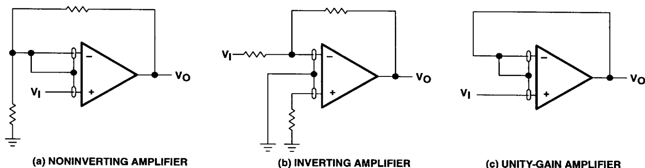
Figure 107. Guard-Ring Schemes
