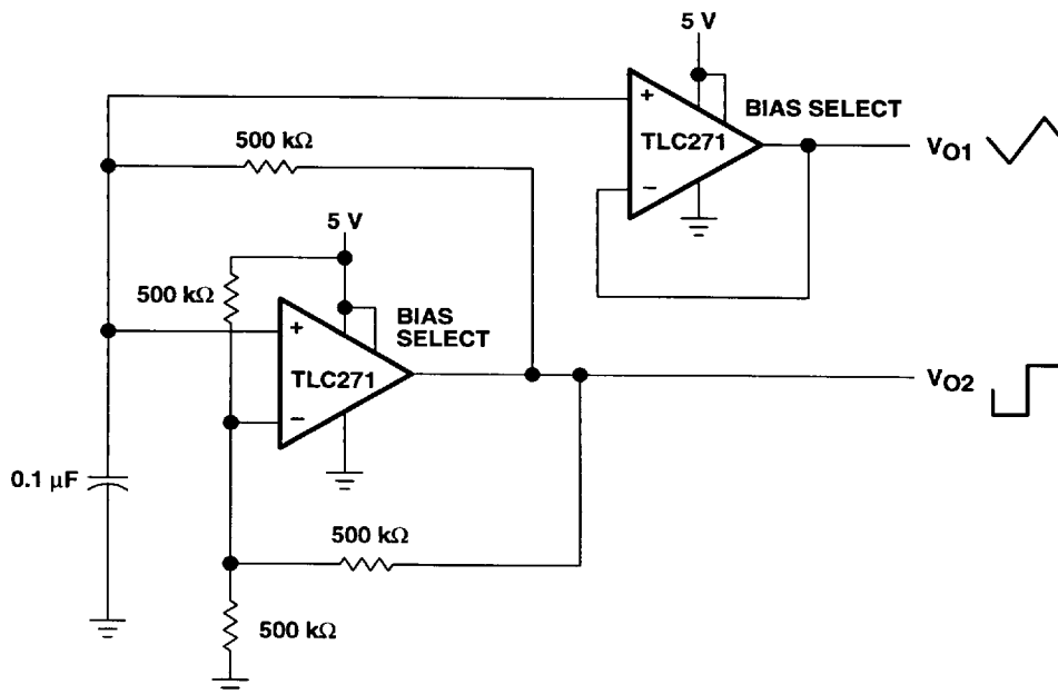
Figure 126. Multivibrator
