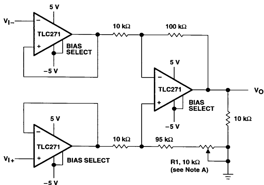
Figure 116. Low-Power Instrumentation Amplifier
