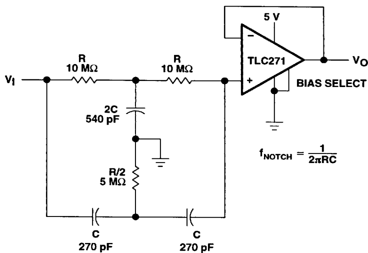
Figure 117. Single-Supply Twin-T Notch Filter
