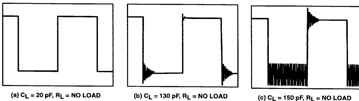
Figure 110. Effect of Capacitive Loads in High-Bias Mode
