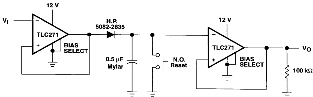
Figure 119. Positive-Peak Detector
