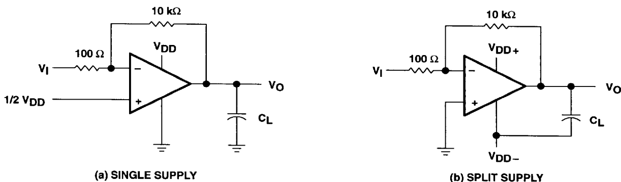
Figure 100. Gain-of-100 Inverting Amplifier
