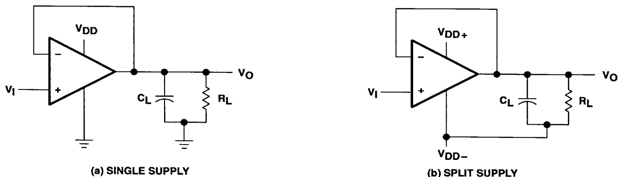
Figure 98. Unity-Gain Amplifier
