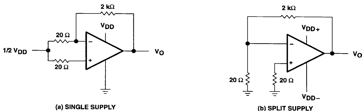
Figure 99. Noise-Test Circuit
