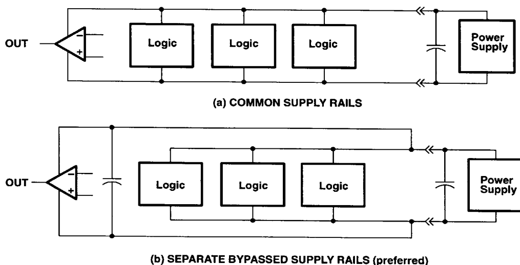
Figure 104. Common Versus Separate Supply Rails
