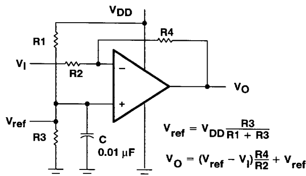
Figure 103. Inverting Amplifier With Voltage Reference
