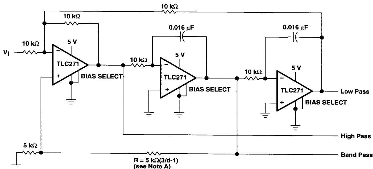
Figure 114. State-Variable Filter
