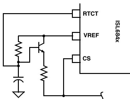
FIGURE 7. SLOPE COMPENSATION
