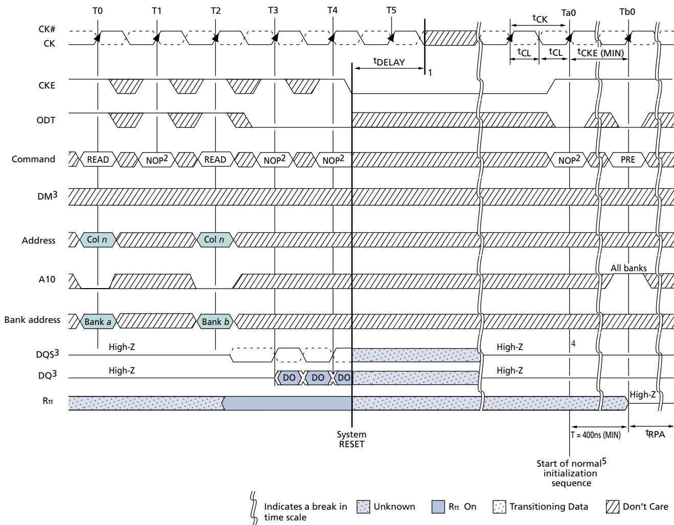
Figure 82: RESET Function
