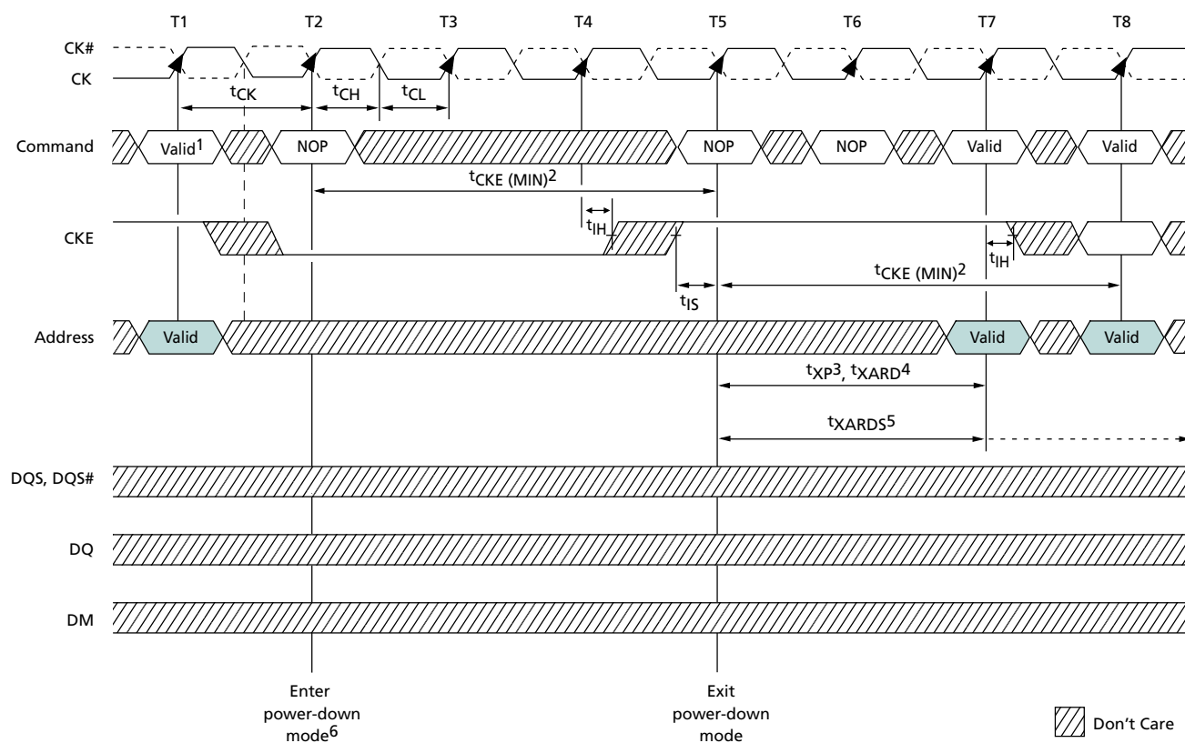
Figure 72: Power-Down
