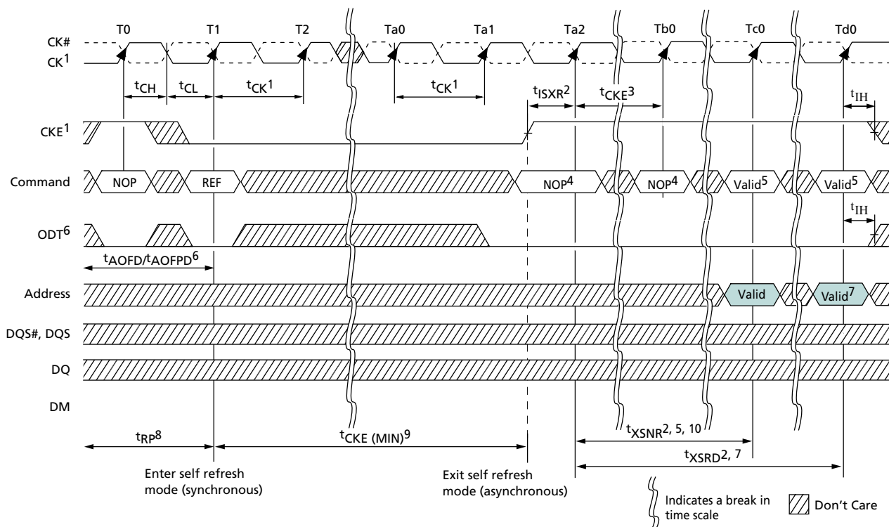
Figure 71: Self Refresh
