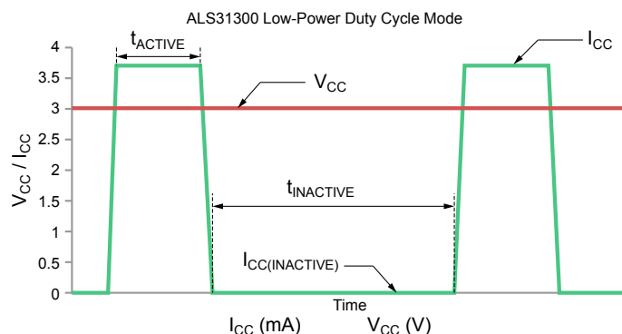
Figure 4: I_{\text{CC}} in Low-Power Duty Cycle Mode
