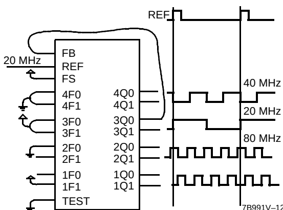
Figure 6. Frequency Multiplier with Skew Connections
