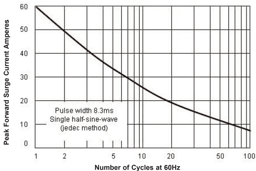
Figure 2 - Maximum Non-repetitive Surge Current
