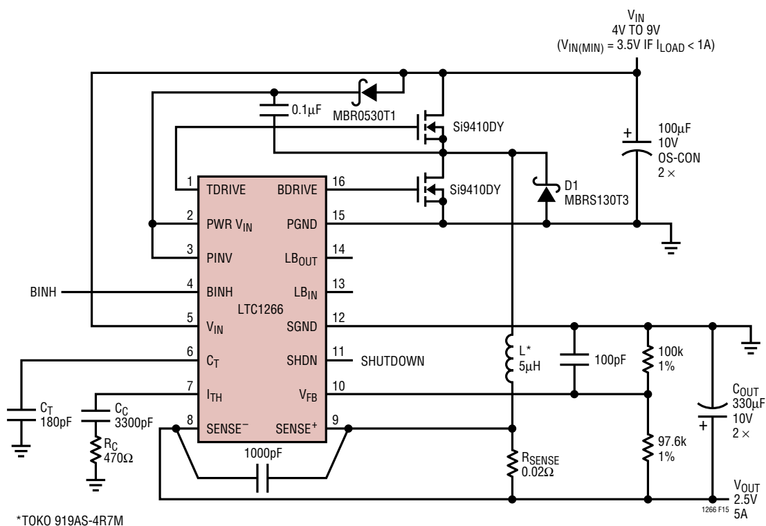
Figure 15. All N-Channel 5V to 2.5V/5A High Efficiency Regulator
