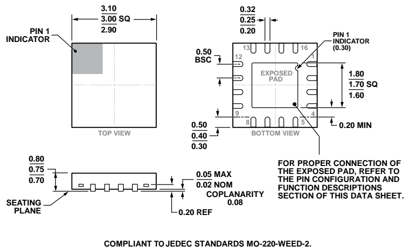
Figure 52. 16-Lead Lead Frame Chip Scale Package [LFCSP_WQ] 3 mm × 3 mm Body, Very Very Thin Quad (CP-16-35)
