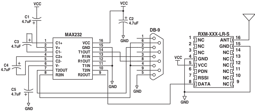
Figure 17: LR Receiver and MAX232 IC
