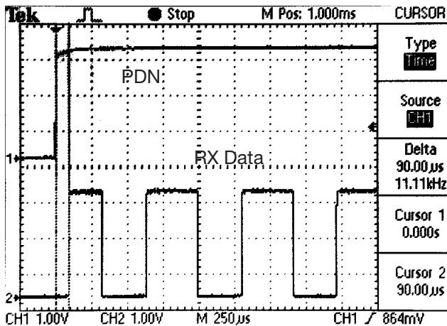
Figure 7: Turn-On Time from PDN
