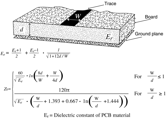
Figure 20: Microstrip Formulas
