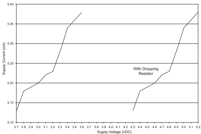
Figure 8: Consumption vs. Supply
