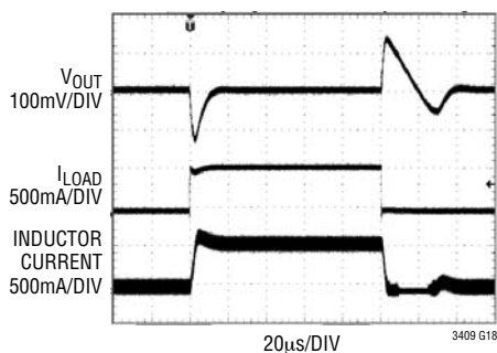
Load Step 50mA to 600mA Pulse Skip
