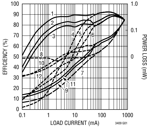
Efficiency/Power Lost vs Load Current, V_{OUT} = 1.8V
