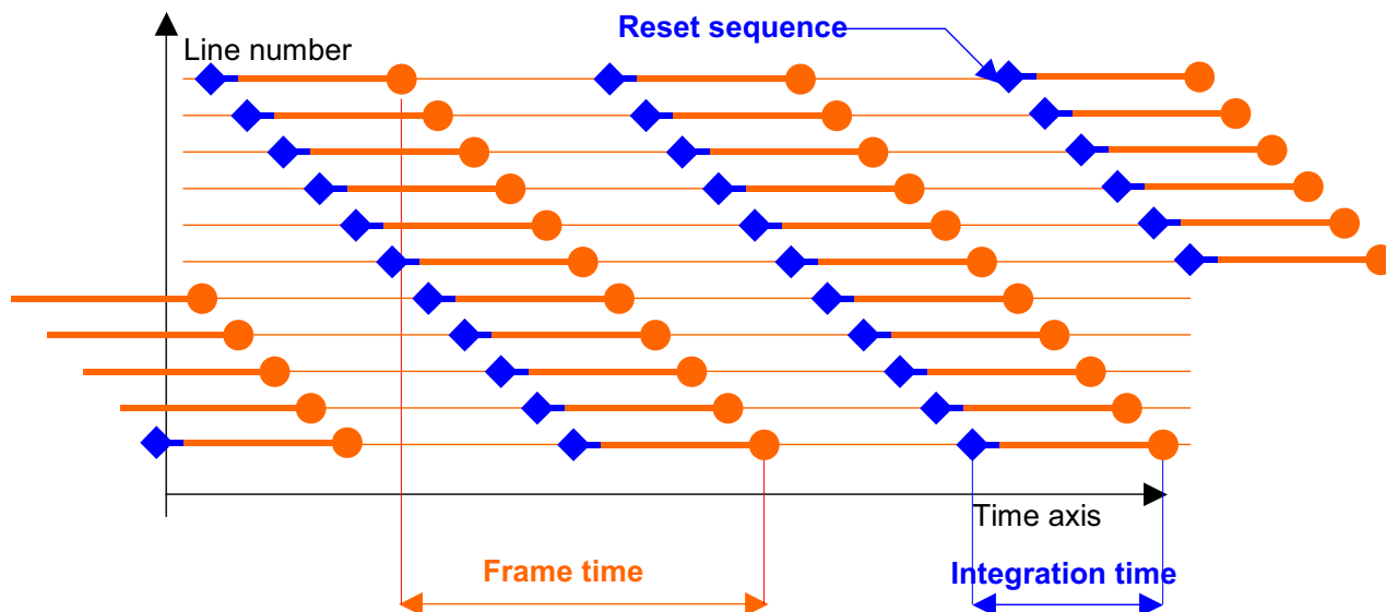
Figure 17. Electronic Rolling Shutter Operation
