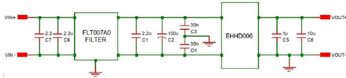
Figure 26. EMC Considerations
