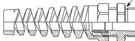
O-Ring Groove
