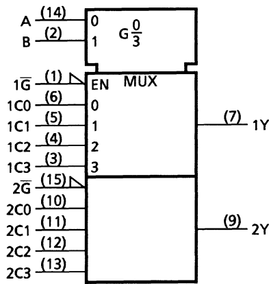
TC74HC153A
