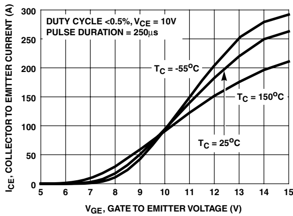
FIGURE 13. TRANSFER CHARACTERISTIC
