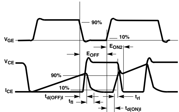
FIGURE 18. SWITCHING TEST WAVEFORMS
