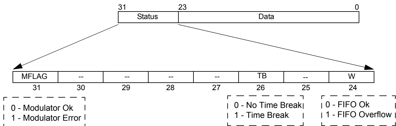
Figure 34. 32-bit Serial Data Format
