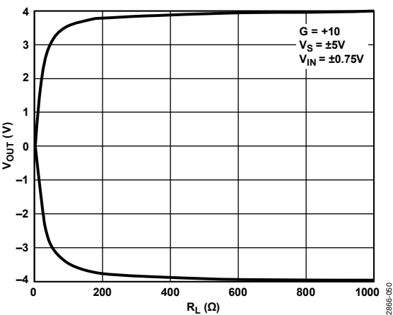
Figure 50. V_{OUT} Swing vs. R_L , V_S = \pm 5V , G = +10 , V_{IN} = \pm 0.75V
