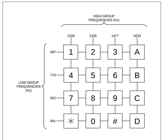
Fig. 6-22 Key Matrix
