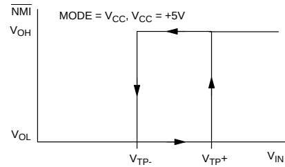
APPLICATION WITH MODE PIN CONNECTED TO V CC Figure 4
