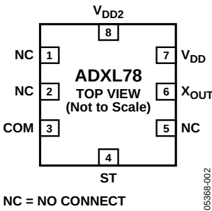
Figure 2. Pin Configuration
