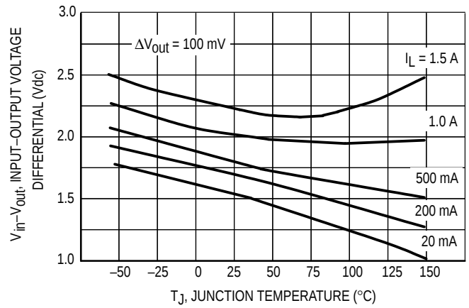
Figure 8. Dropout Voltage
