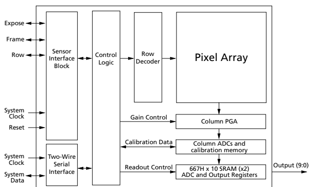
Figure 1: Block Diagram
