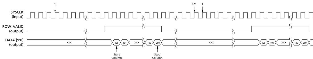
Figure 23: Row Timing for Master Mode and Snapshot Mode with Windowing
