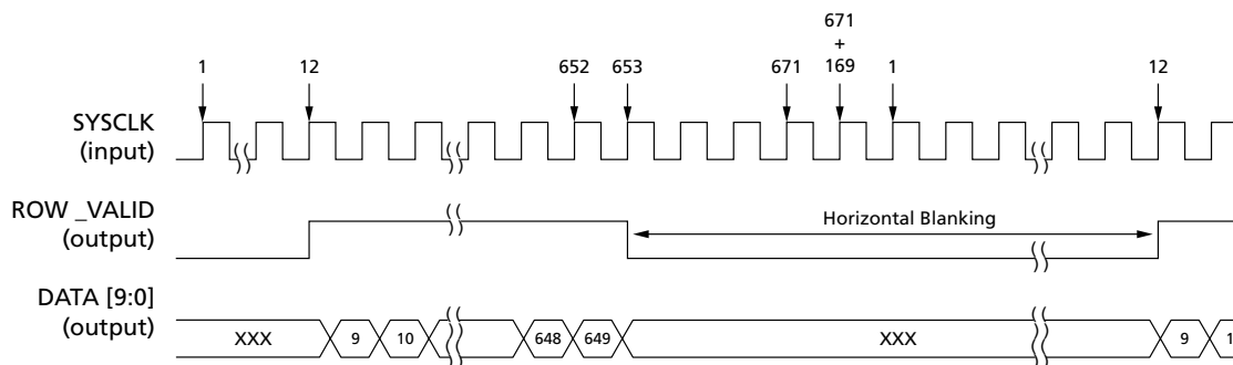
Figure 5: Master Mode Row Timing Diagram
