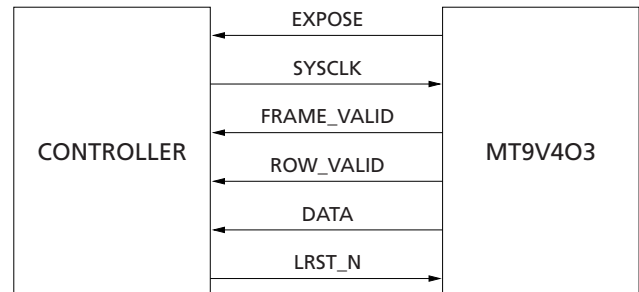
Figure 4: Master Mode Interface Signals
