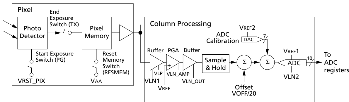
Figure 21: Signal Path
