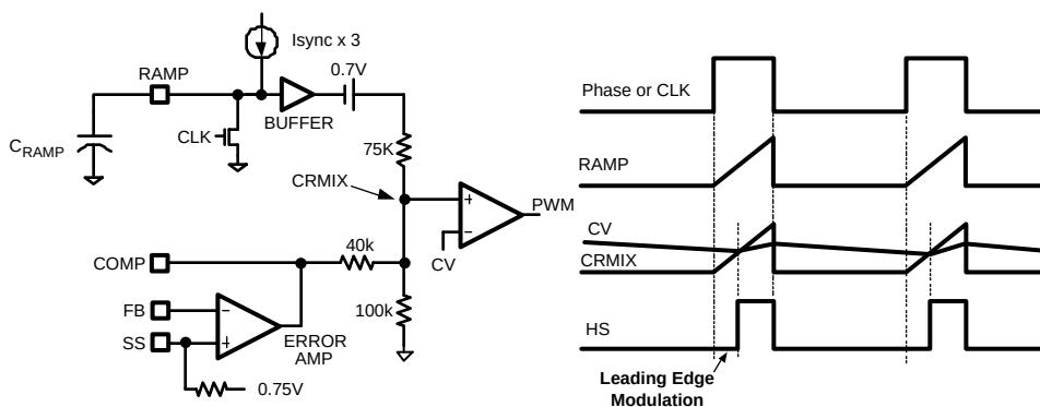
Figure 13. Synchronization and Leading Edge Modulation
