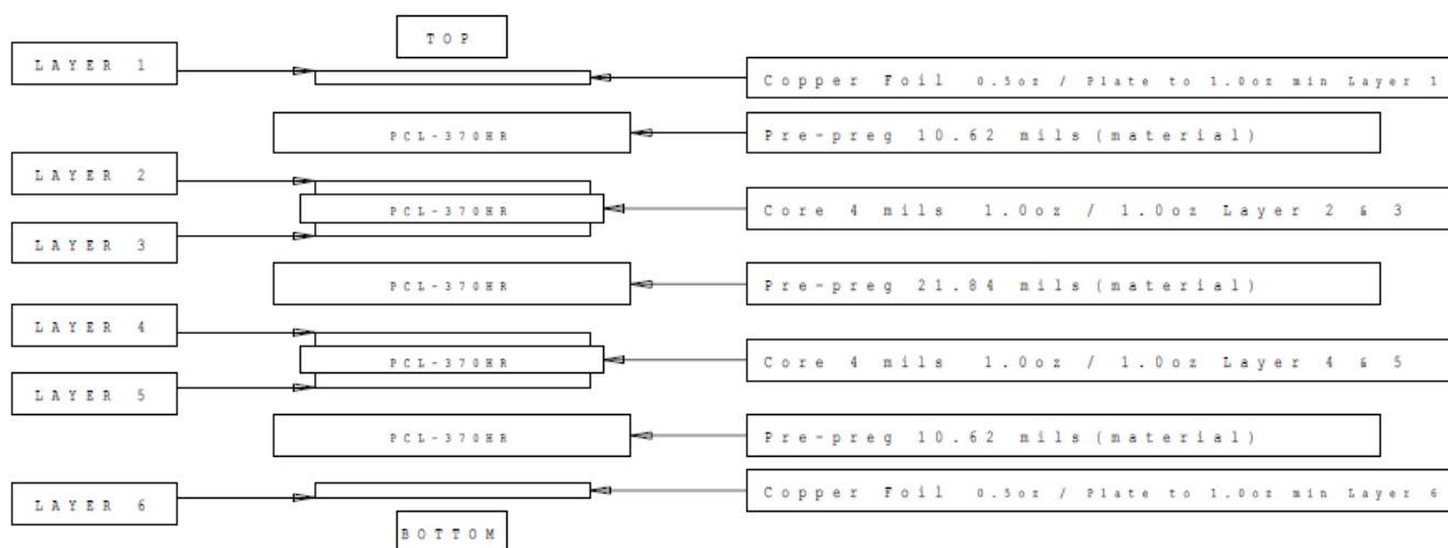
Figure 10. Stackup
