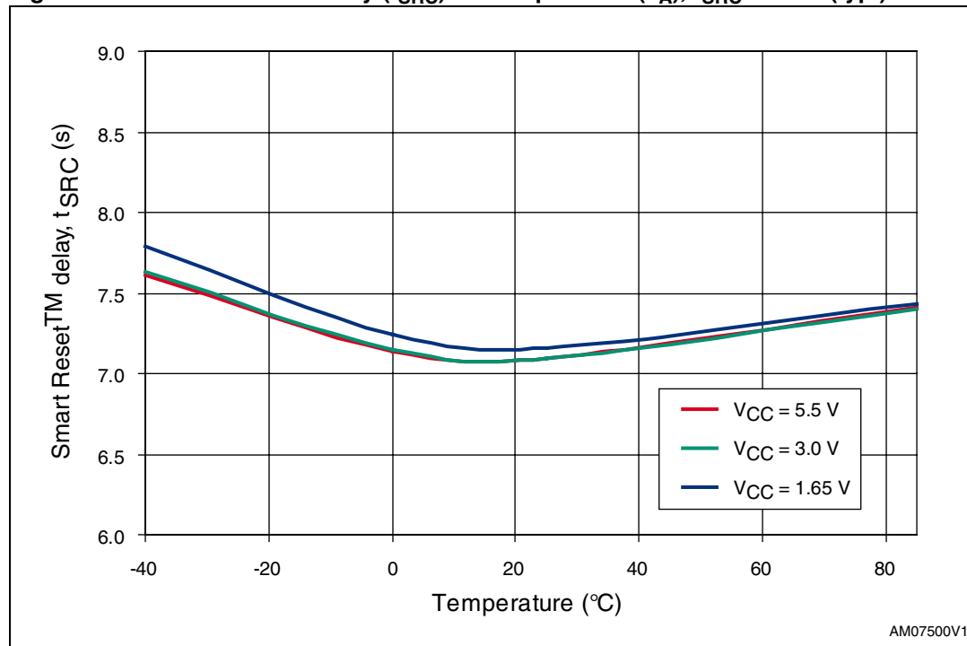
Figure 10. Smart Reset TM delay ( t_{SRC} ) vs. temperature ( T_A ), t_{SRC} = 7.5 s (typ.)
