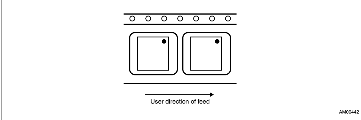
Figure 16. Pin 1 orientation
