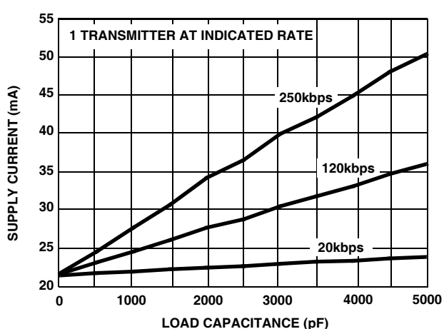
FIGURE 20. ISL4238E SUPPLY CURRENT vs LOAD CAPACITANCE WHEN TRANSMITTING DATA
