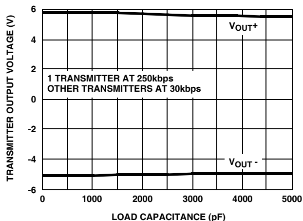
FIGURE 18. ISL4244E TRANSMITTER OUTPUT VOLTAGE vs LOAD CAPACITANCE
