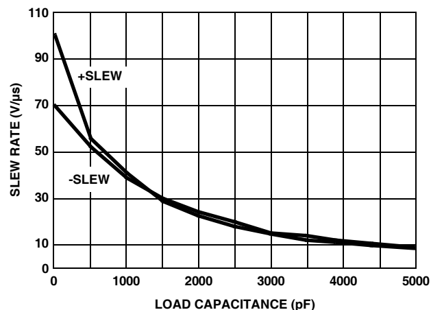
FIGURE 24. ISL4245E SLEW RATE vs LOAD CAPACITANCE
