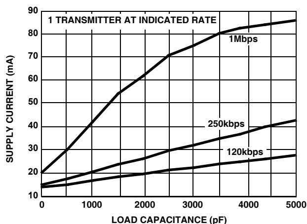
FIGURE 22. ISL4245E SUPPLY CURRENT vs LOAD CAPACITANCE WHEN TRANSMITTING DATA
