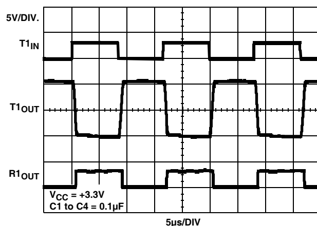
FIGURE 13. ISL4238E/ISL4244E LOOPBACK TEST AT 120kbps
