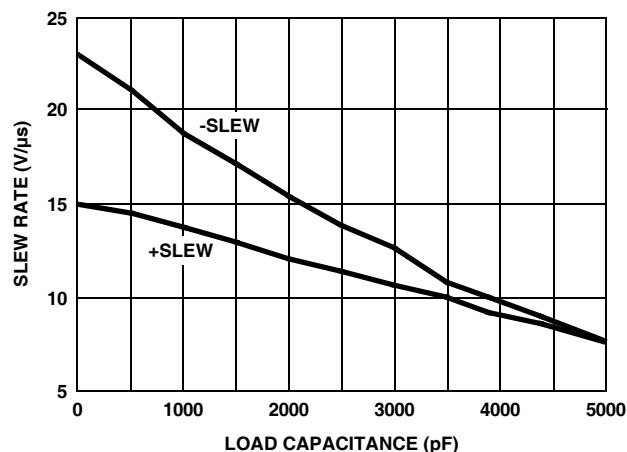
FIGURE 23. ISL4238E/ISL4244E SLEW RATE vs LOAD CAPACITANCE
