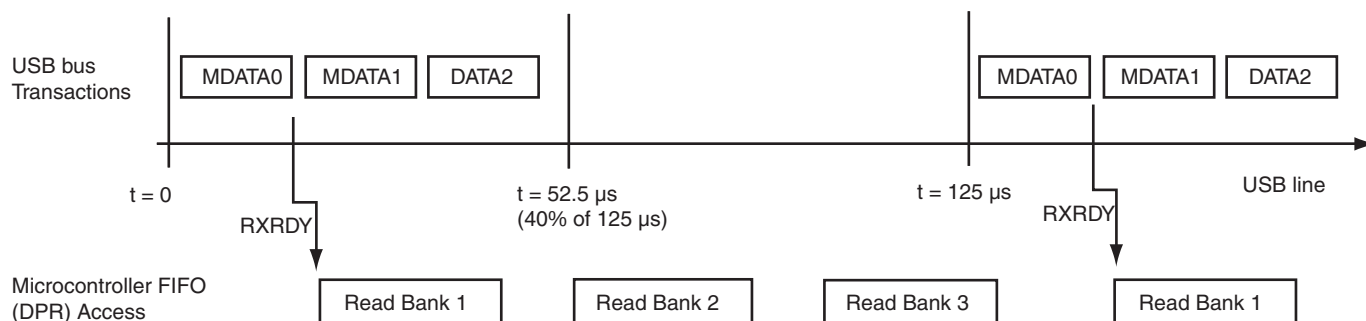
Figure 32-16.Bank Management, Example of Three Transactions per Microframe
