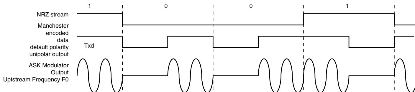
Figure 39-18.ASK Modulator Output
