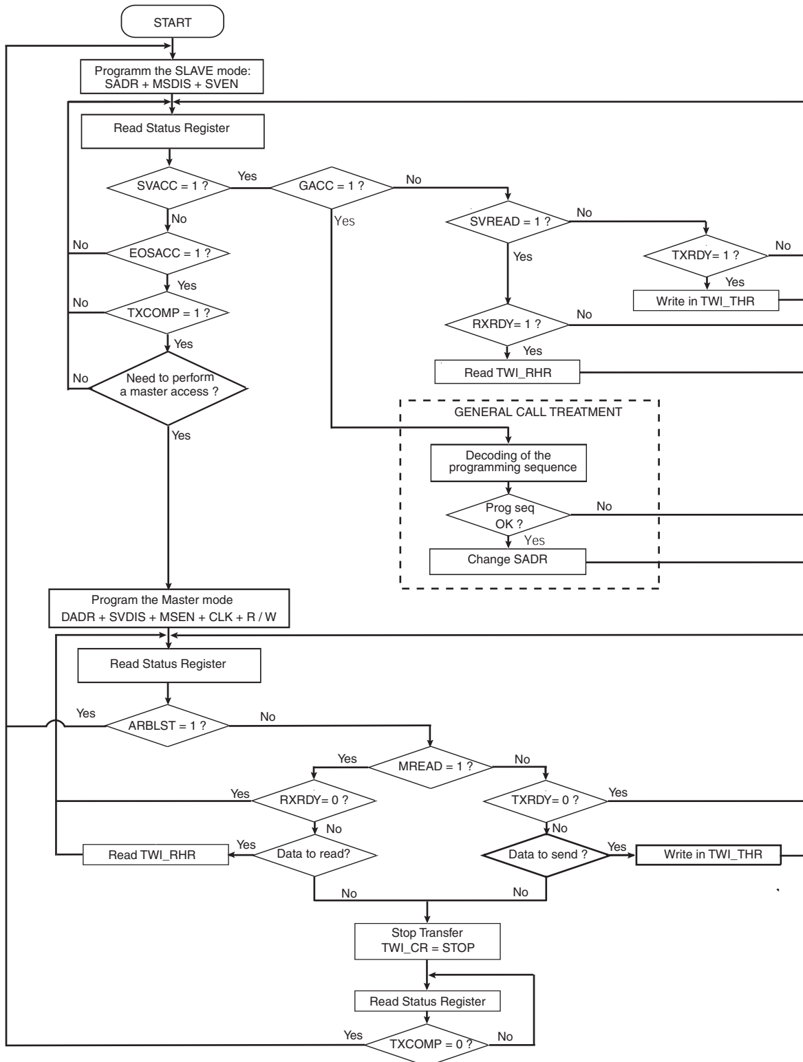
Figure 38-24. Multi-master Flowchart
