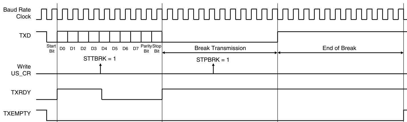
Figure 39-26. Break Transmission
