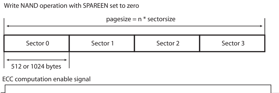
Figure 27-4. NAND Write Operation
