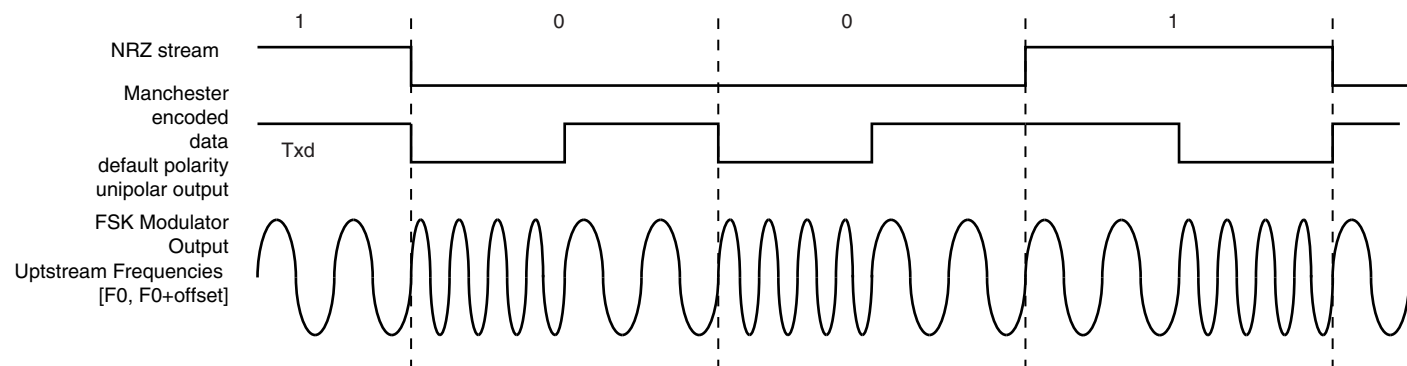
Figure 39-19.FSK Modulator Output
