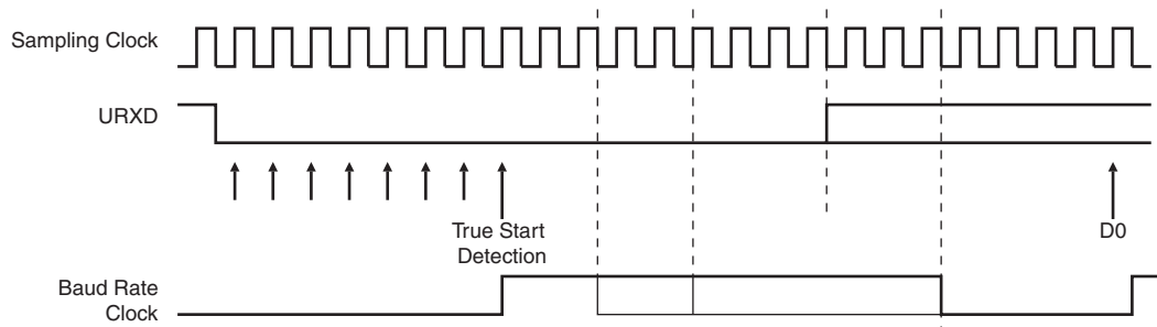
Figure 40-3. Start Bit Detection
