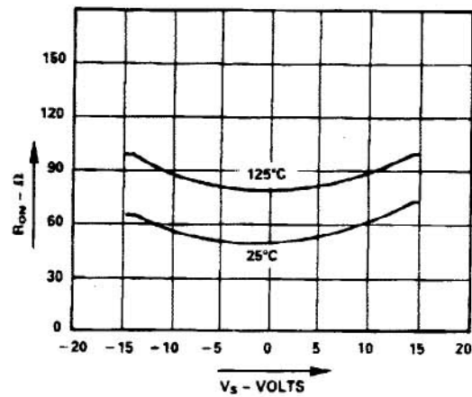
R_{ON} AS A FUNCTION OF V_S ( V_D ) FOR DIFFERENT TEMPERATURES
