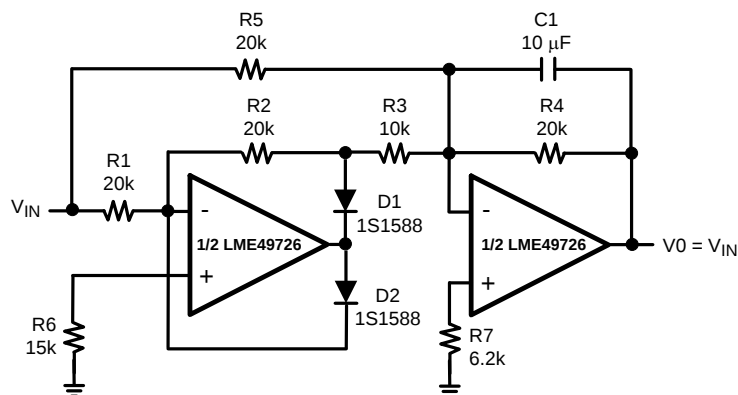
Figure 41. AC/DC Converter
