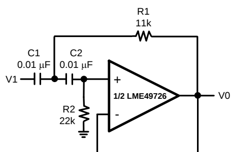
Figure 37. Sine Wave Oscillator
