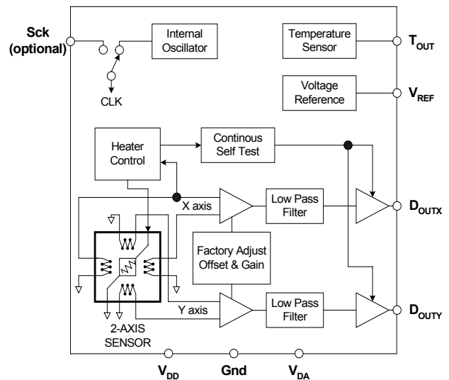
MXD2020U/W FUNCTIONAL BLOCK DIAGRAM
