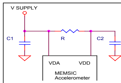
Figure 8: Power Supply Noise Rejection
