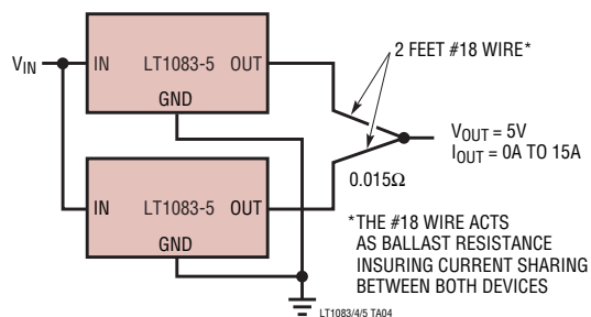
Paralleling Regulators
