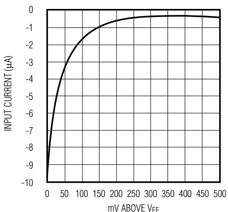
Figure 4. Enable Logic-Low Input Current vs. V_{IL} with 10kΩ Series Resistor
