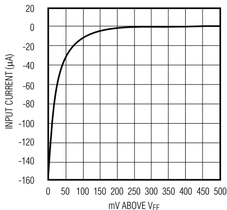
Figure 2. Enable Logic-Low Input Current vs. V_{IL}
