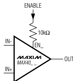
Figure 3. Circuit to Reduce Enable Logic-Low Input Current
